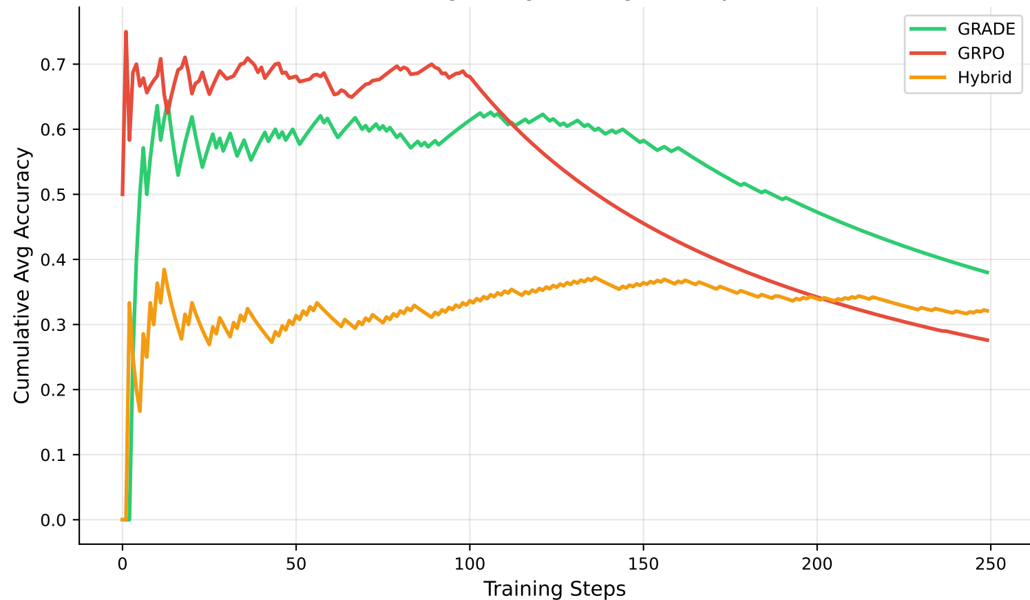
Running Average Training Accuracy
